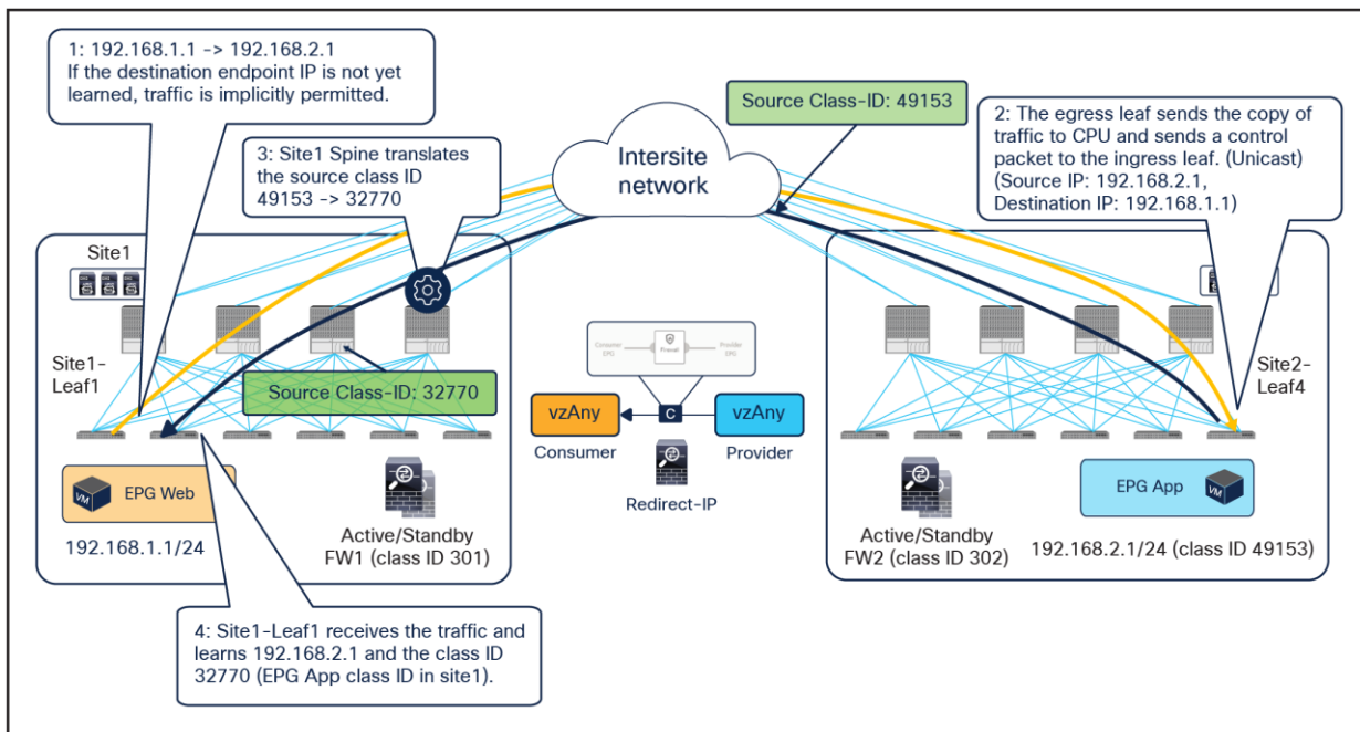
Figure 139. Conversational learning for endpoint-to-endpoint communication (unicast)
