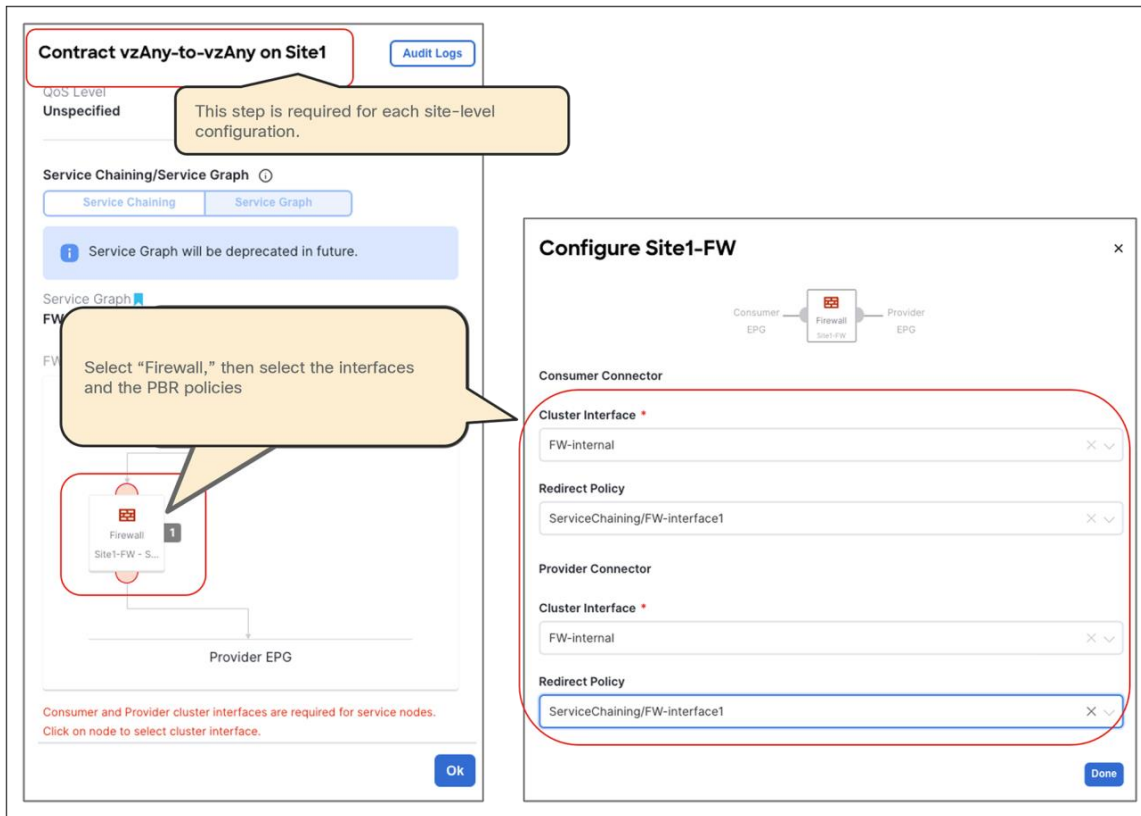
Figure 185. Select interfaces and PBR policies (site-level)
