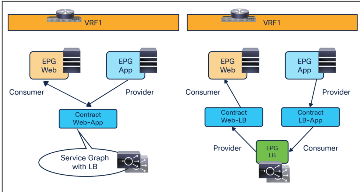
Figure 43. Load-balancer insertion with (left) and without (right) service graph
