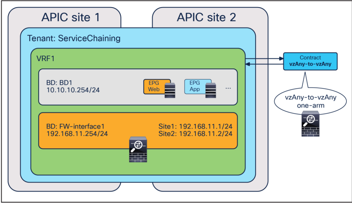
Figure 113. vzAny-to-vzAny contract with PBR
