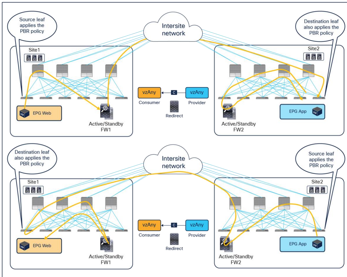
Figure 24. Use of ACI PBR to keep intersite traffic symmetric for the vzAny-to-vzAny PBR use case
