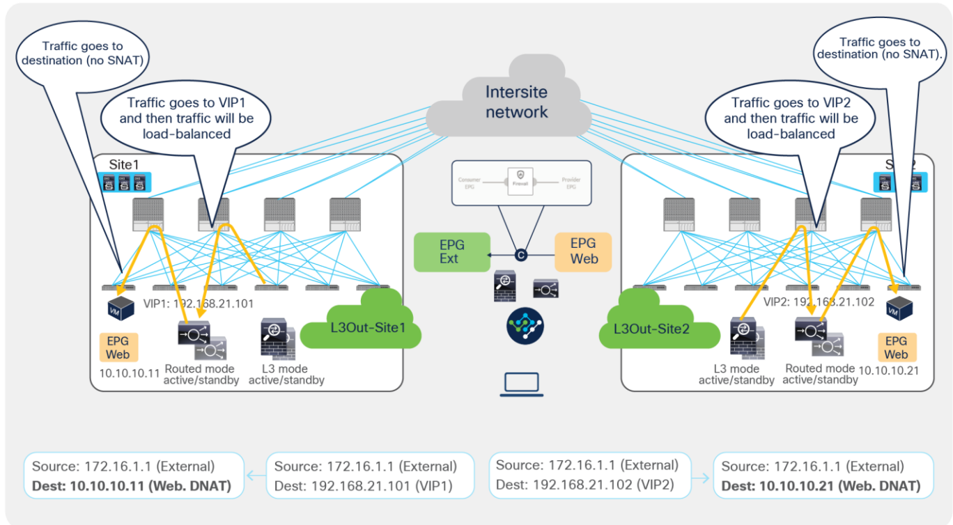
Figure 65. Firewall with PBR and load balancer without SNAT inbound traffic flows (VIP to real-servers)
