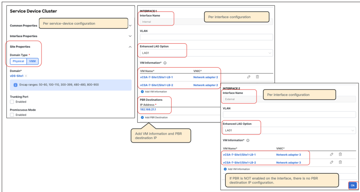
Figure 98. Example of a load-balancer configuration (two-arm, site-level with VMM domain)
