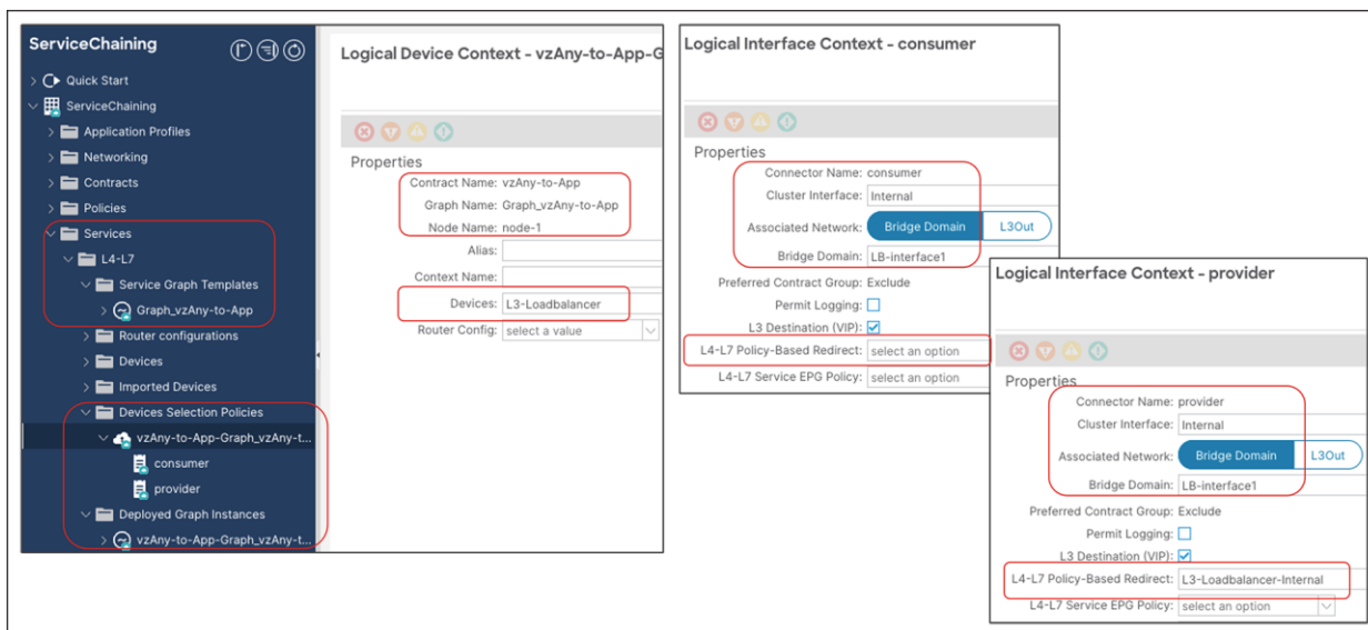
Figure 126. Verify the configuration on APIC (Device Selection Policy and Deployed Graph Instance)
