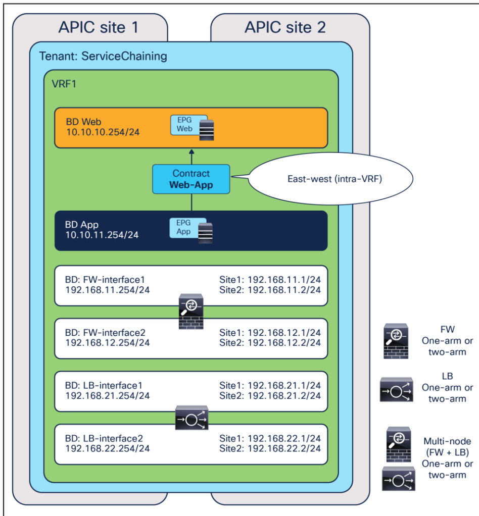
Figure 100. EPG-to-EPG contract with PBR (intra-VRF)
