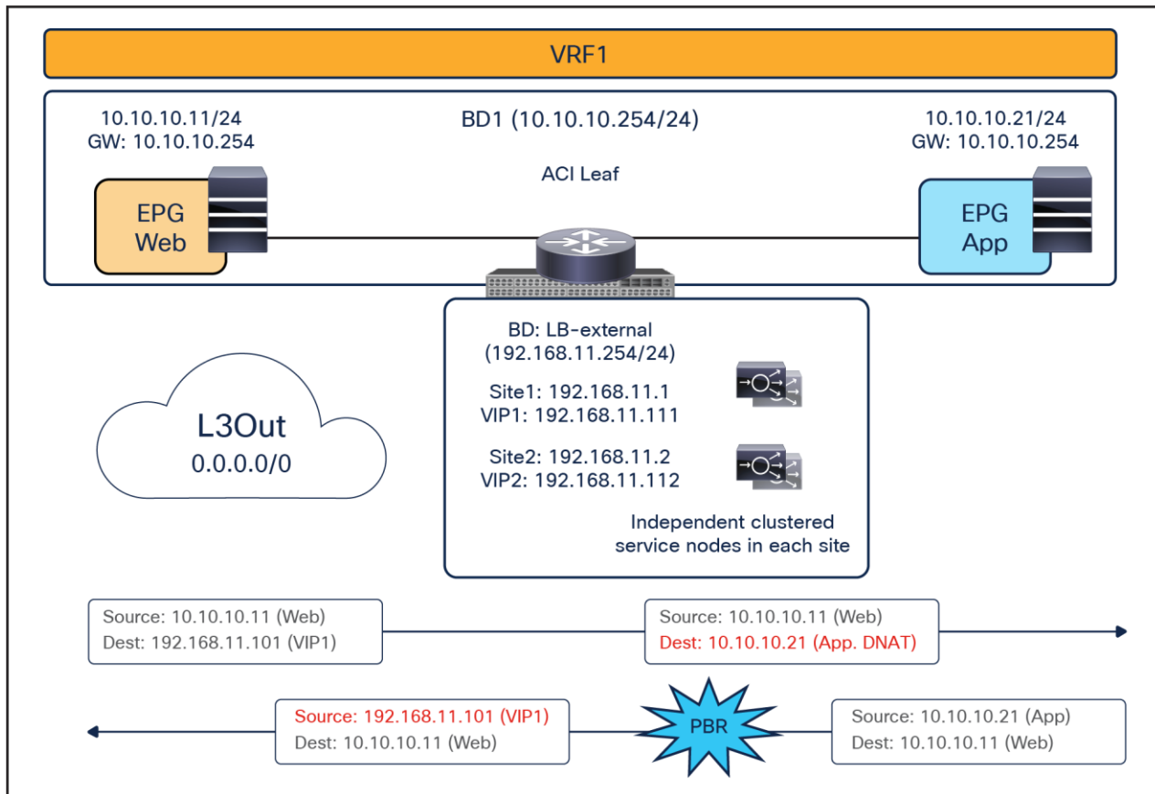
Figure 60. Example of east-west and north-south load balancer without a SNAT design
