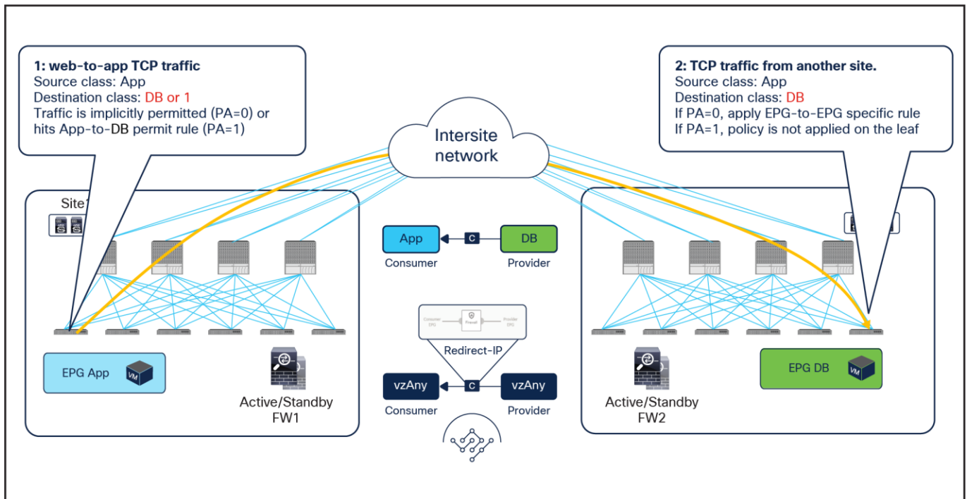
Figure 74. Specific EPG-to-EPG rule wins over vzAny-to-vzAny rule
