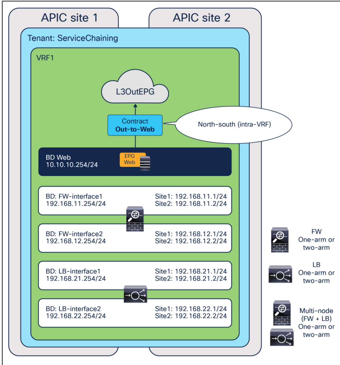
Figure 108. L3Out-to-EPG contract with PBR (intra-VRF)
