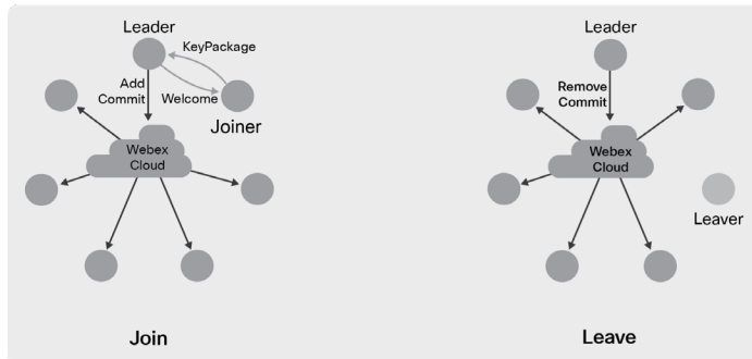
Figure 7. Group key management with MLS
