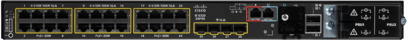
Figure 4. IE-9320-24P4S Switch
