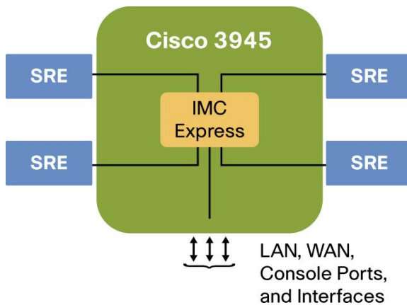
Figure 10. Cisco IMC Express Architecture for Cisco 3945 ISR
