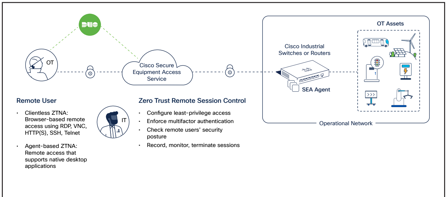
Figure 1. Cisco Secure Equipment Access's ZTNA architecture
