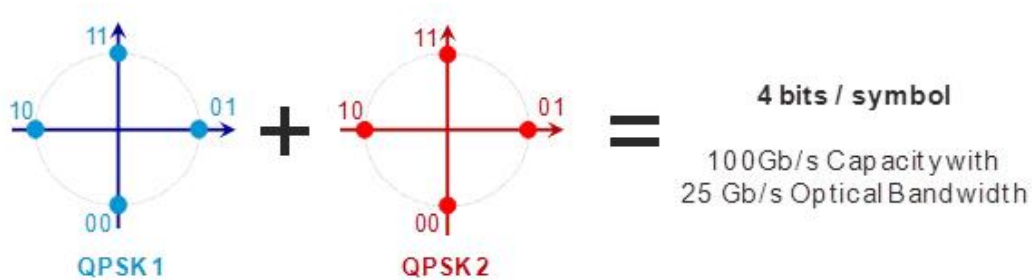
Figure 3. CP-DQPSK Logical Transmitter Scheme
