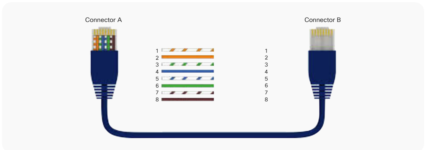
Figure 5. Straight cable
