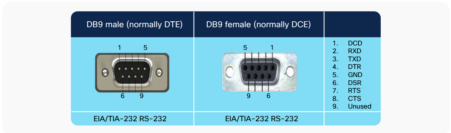
Figure 4. DB9 connector
