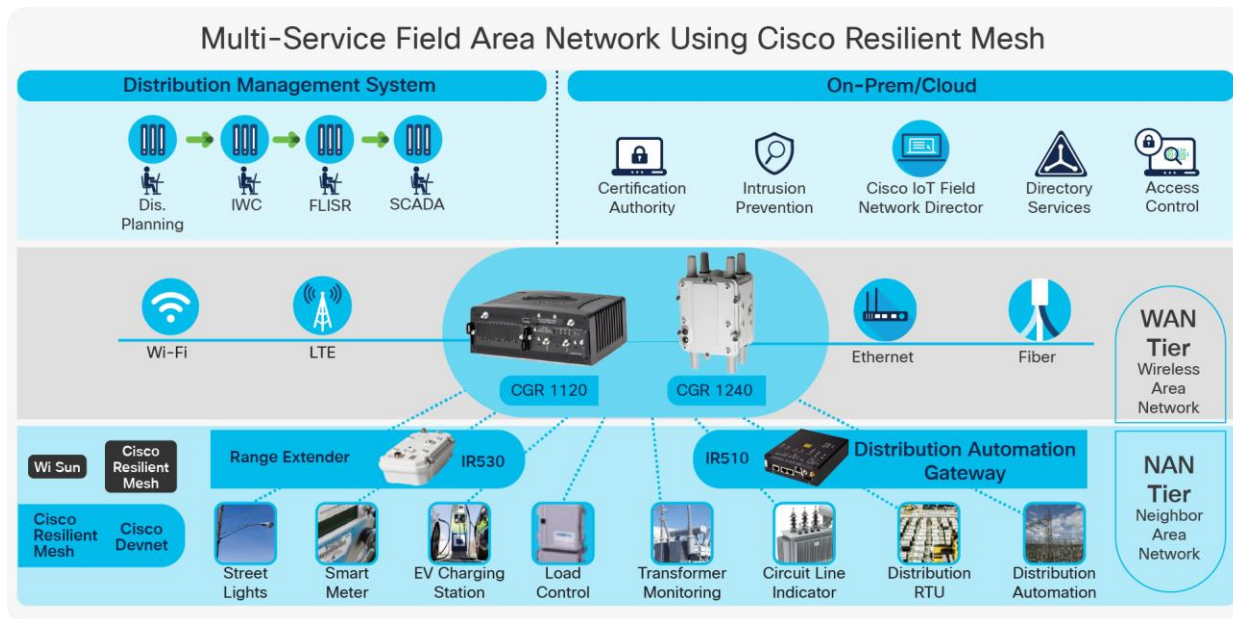
Figure 2. Cisco Connected Grid FAN solution
