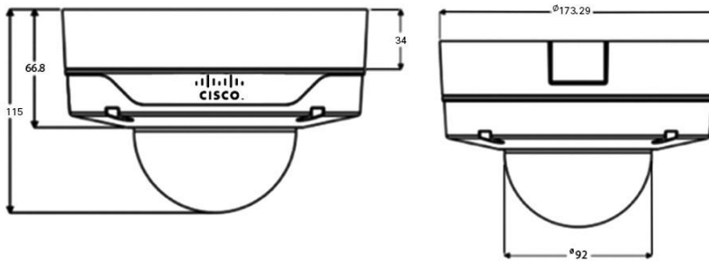
Figure 2. Cisco Video Surveillance 3530 IP Camera Dimensions
