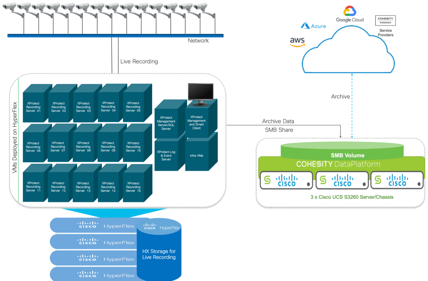
Figure 5. Logical topology
