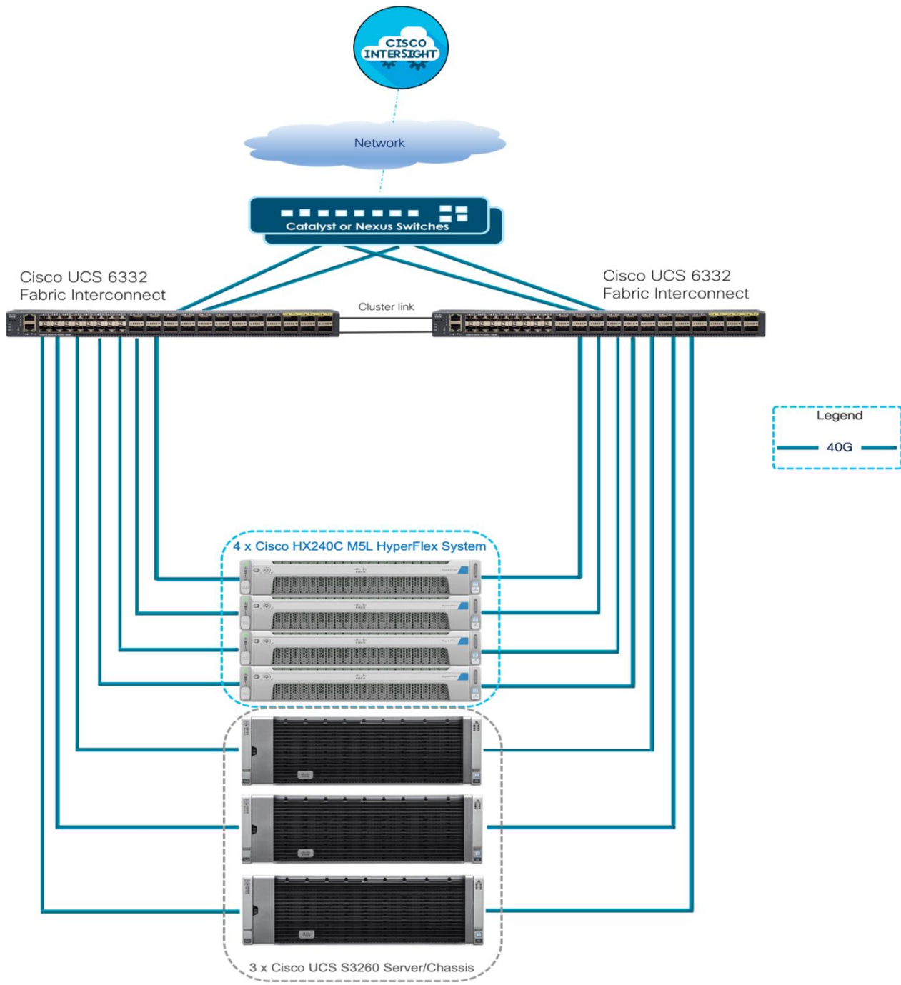
Figure 4. Physical topology
