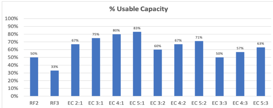
Figure 18. Usable capacity based on replication factor and erasure coding
