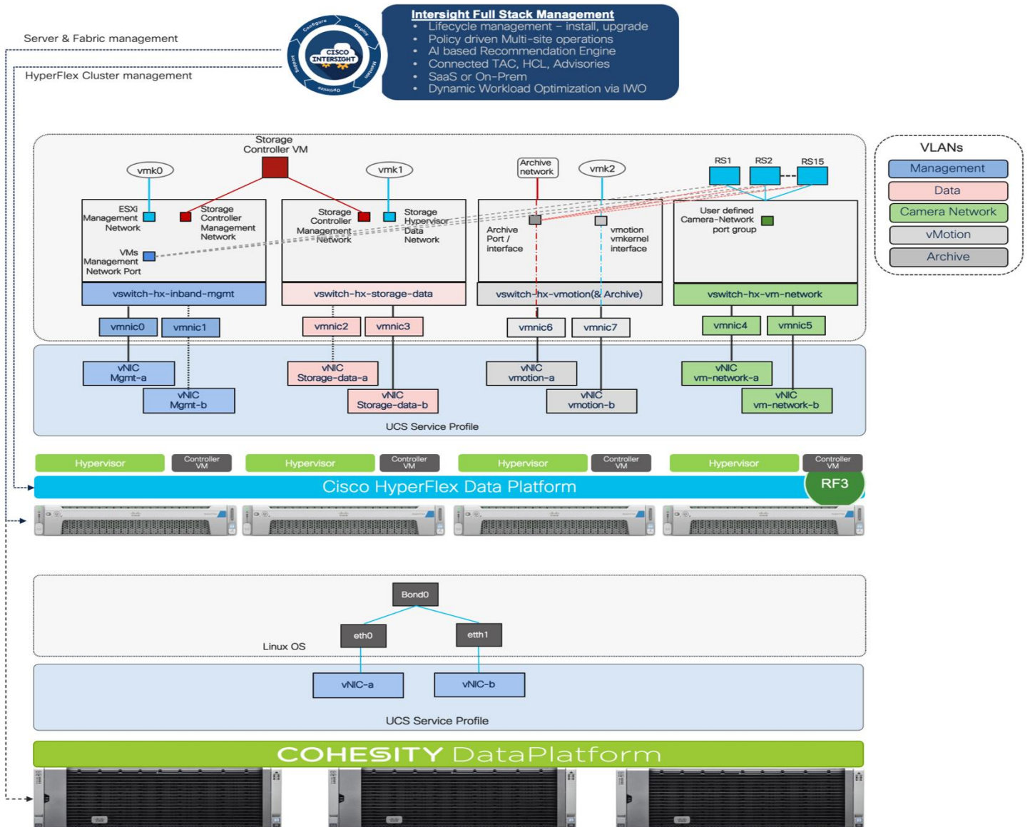
Figure 6. Logical network layout
