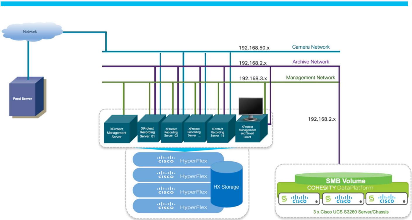
Figure 7. Virtual machine and port group mappings
