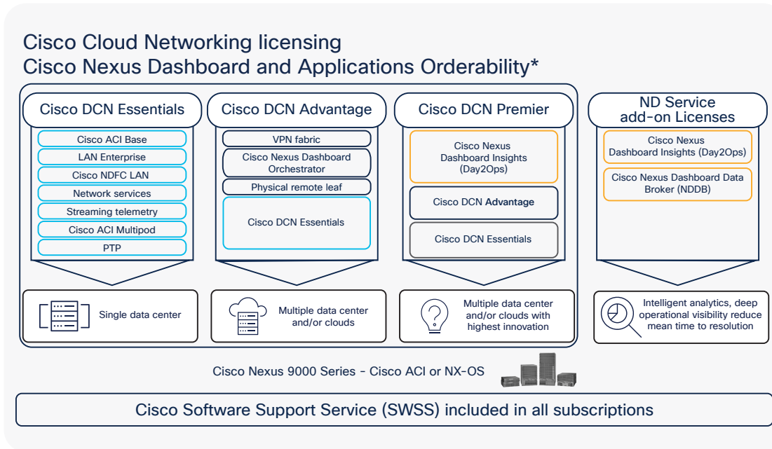
Figure 1. Licensing overview
