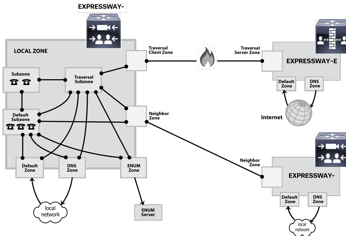
Figure 14 Example network diagram
