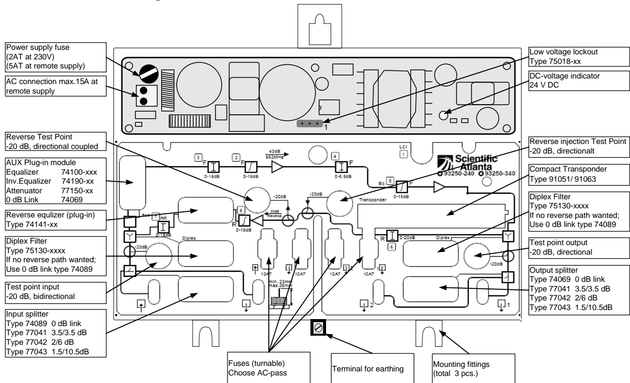
Figure 1: Amplifier overview
