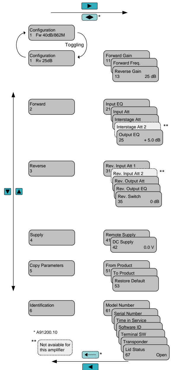
Figure 3. Menu Structure
