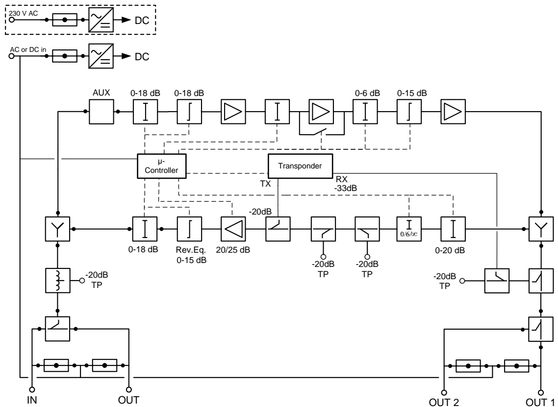
Figure 2: Block diagram for the amplifier type 93250
