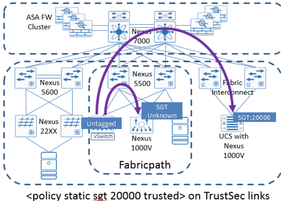
Figure 12 Link behavior with untagged traffic
