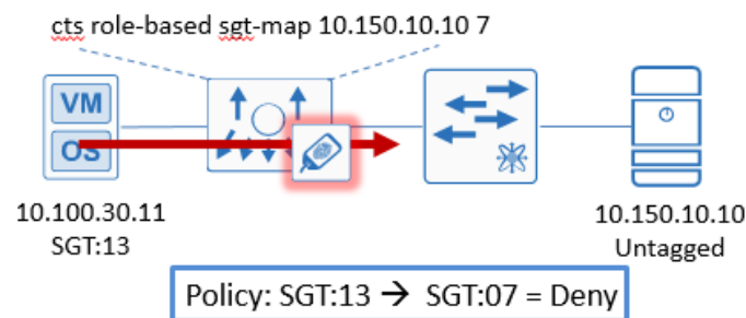
Figure 21 Nexus 1000V and Static IP-SGT or SXP mappings
