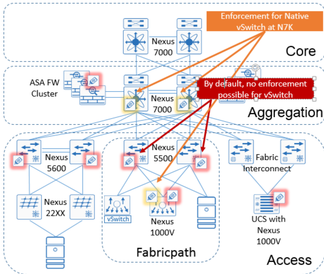
Figure 58 Sample network policy enforcement
