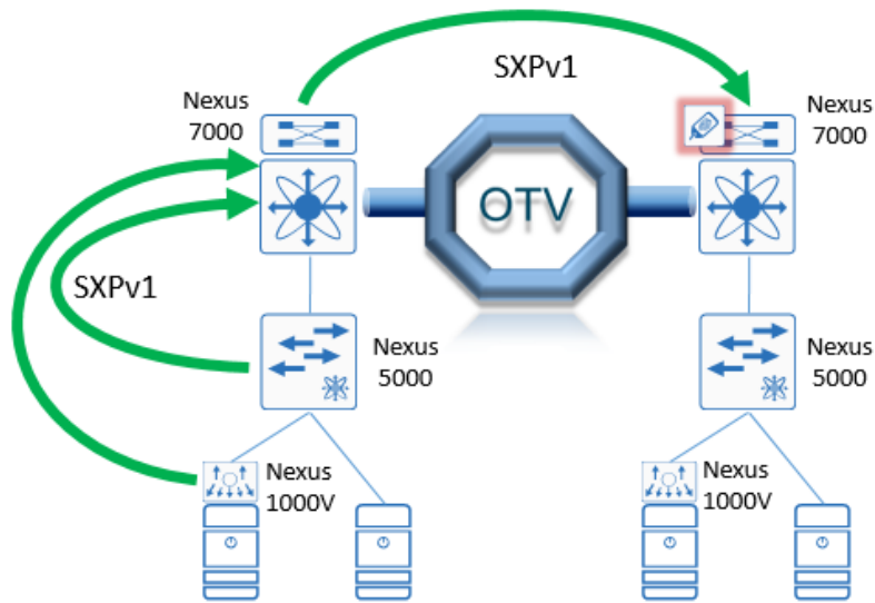
Figure 15 SXP over OTV between data centers
