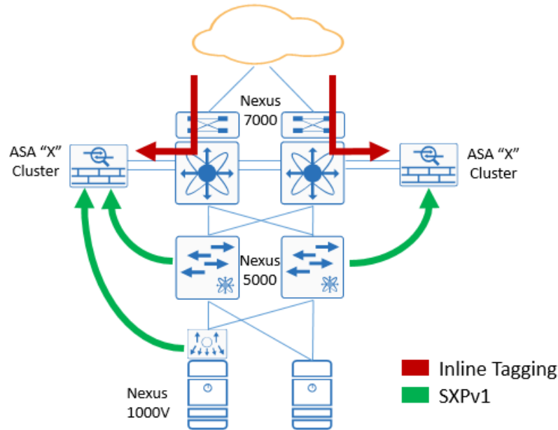
Figure 16 SXP use with ASA Cluster in the data center
