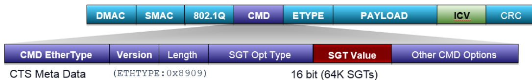
Figure 1 Layer 2 Frame with Cisco Meta Data field containing SGT
