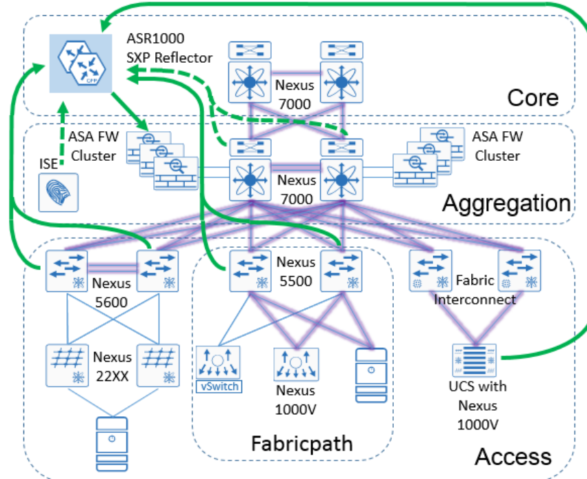
Figure 57 TrustSec propagation in the sample Data Center
