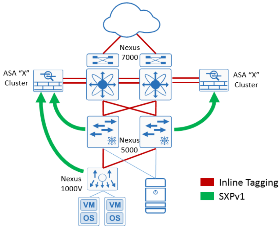
Figure 29 ASA SGFW using SXP and inline tagging
