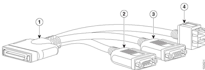
Figure 17 KVM Cable
