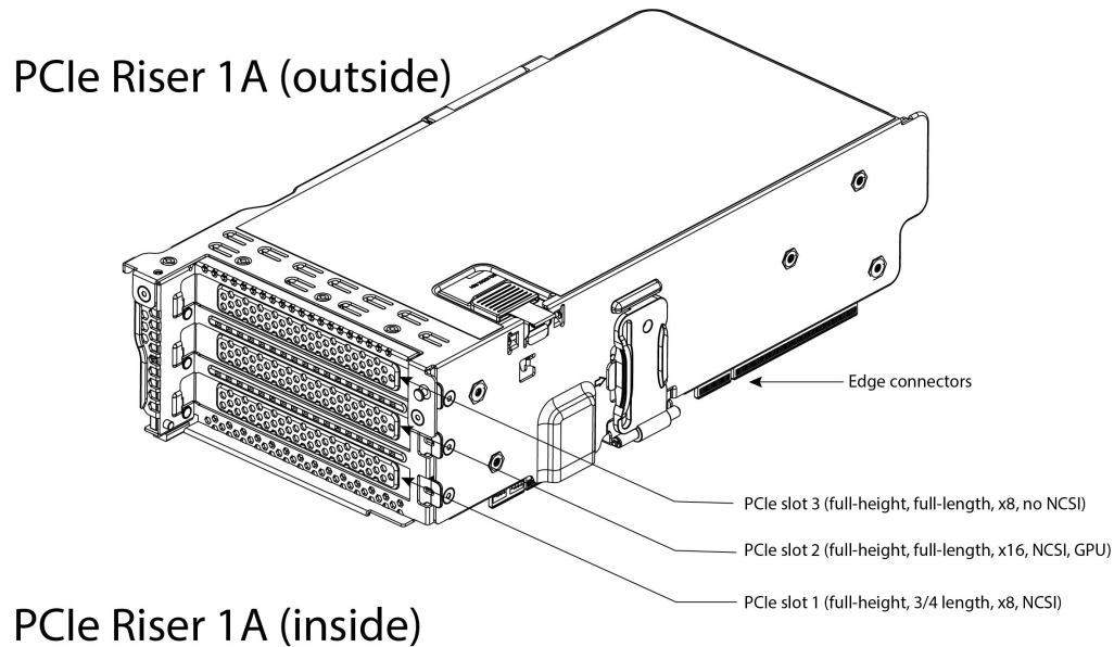
Figure 21 Riser Card 1A
