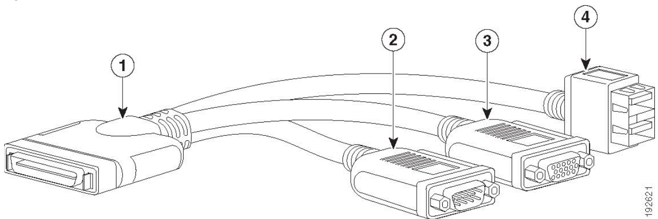
Figure 13 KVM Cable
