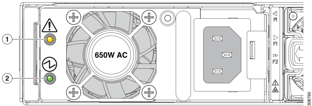
Figure 4 AC Power Supply for the Cisco UCS 6454 Fabric Interconnect
